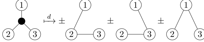
Figure 29: The differential of \text{Tw Gra}_n . This particular example shows that the Arnold relation (the RHS) is killed up to homotopy.
