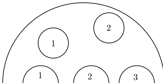
Figure 2.1: Example of an element in \mathbf{SC}(3, 2)
